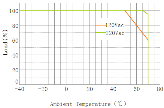
Derating Curve
